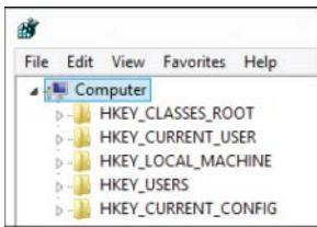
FIGURE 14.13 Windows registry.
