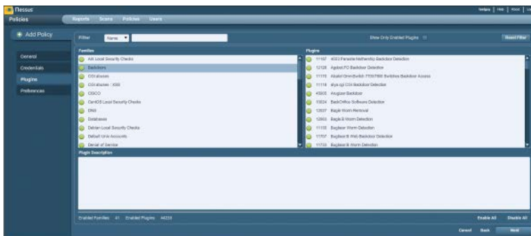
FIGURE 11.13 Selecting plug-ins.
