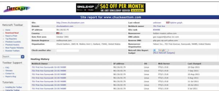
FIGURE 6.1 www.netcraft.com.
